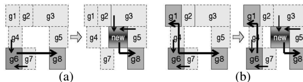
Fig. 1. Example transformations for row-based standard-cell layout: (a) resynthesized gate new replaces g_6 to drive g_8 , (b) gate cloning uses resynthesized gate new to drive g_8 , while the original driver g_6 continues to drive g_1 .
